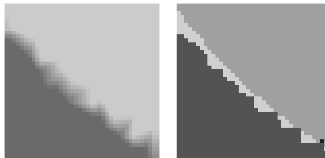
Figure 6. Fragment of the test image upsampled by factor of four using the proposed stochastic method and its difference image.
